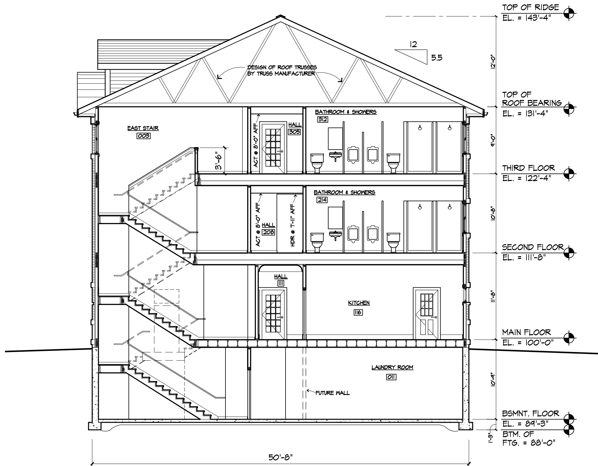
C EAST LOOKING SECTION SCALE: 1/8" = 1'-0" DATE 03-23-2012 O+A JOB# 0532
